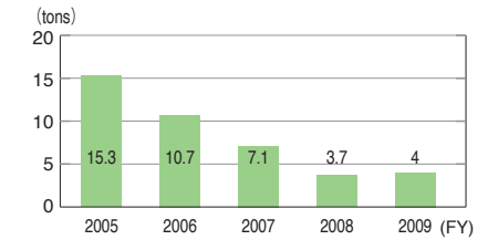
Trends in soot and dust emissions *4
